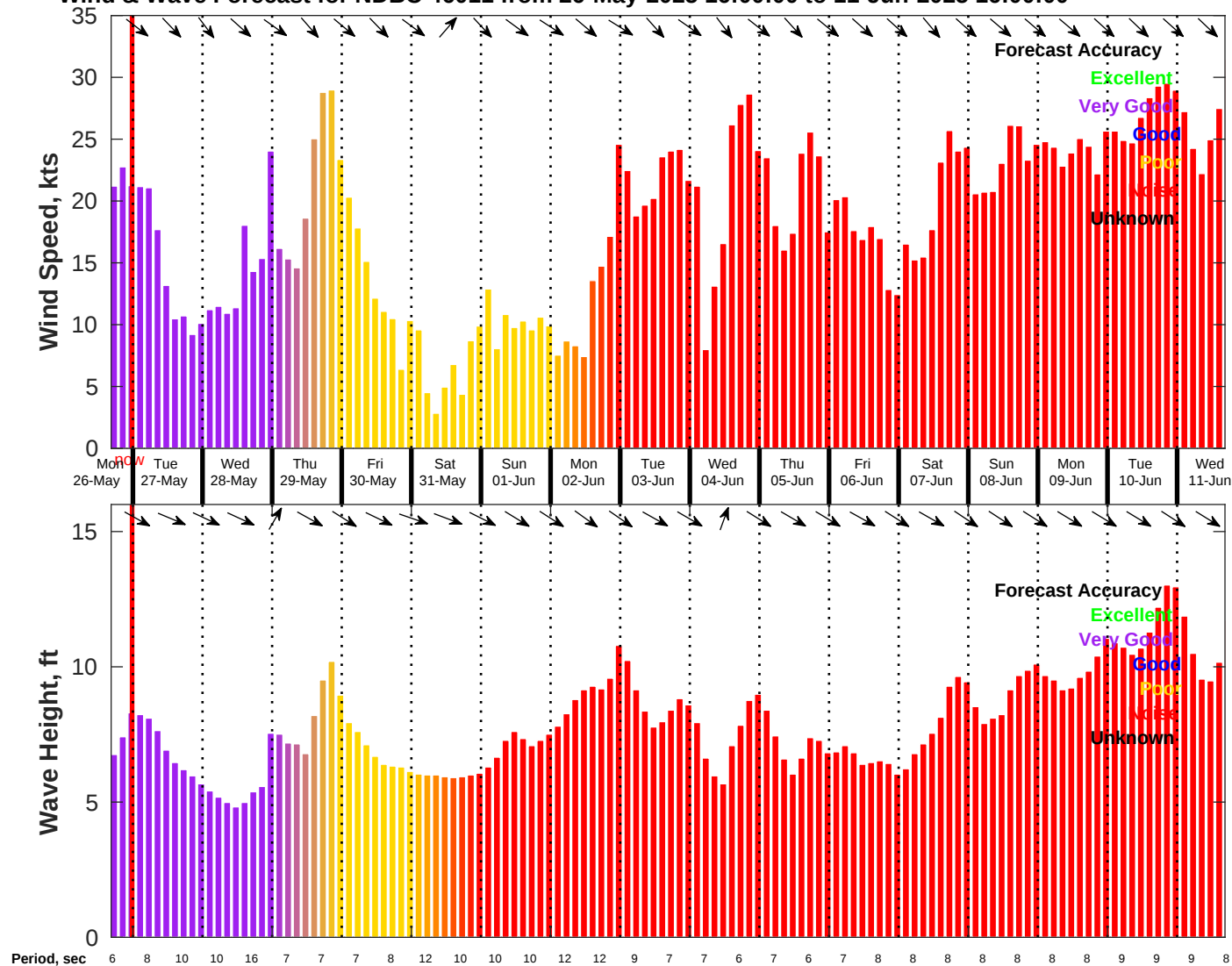
Wind & Wave Forecast for NDBC 46011 from 26-May-2025 16:00:00 to 11-Jun-2025 16:00:00
