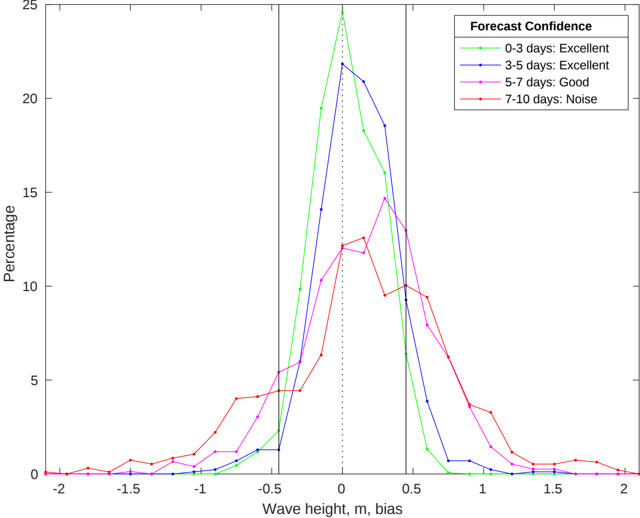
NDBC 46028 vs CMEMS Waves Bias Histogram: 27-May-2025
