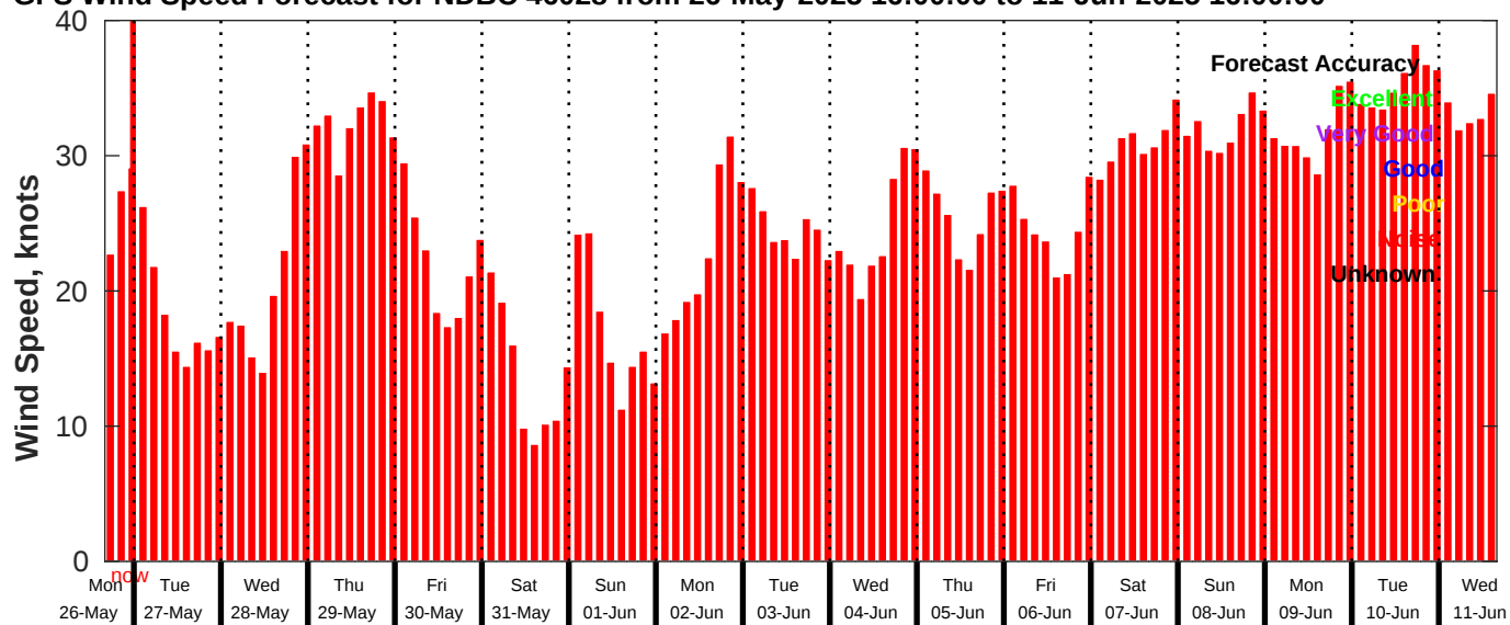
GFS Wind Speed Forecast for NDBC 46028 from 26-May-2025 16:00:00 to 11-Jun-2025 16:00:00
