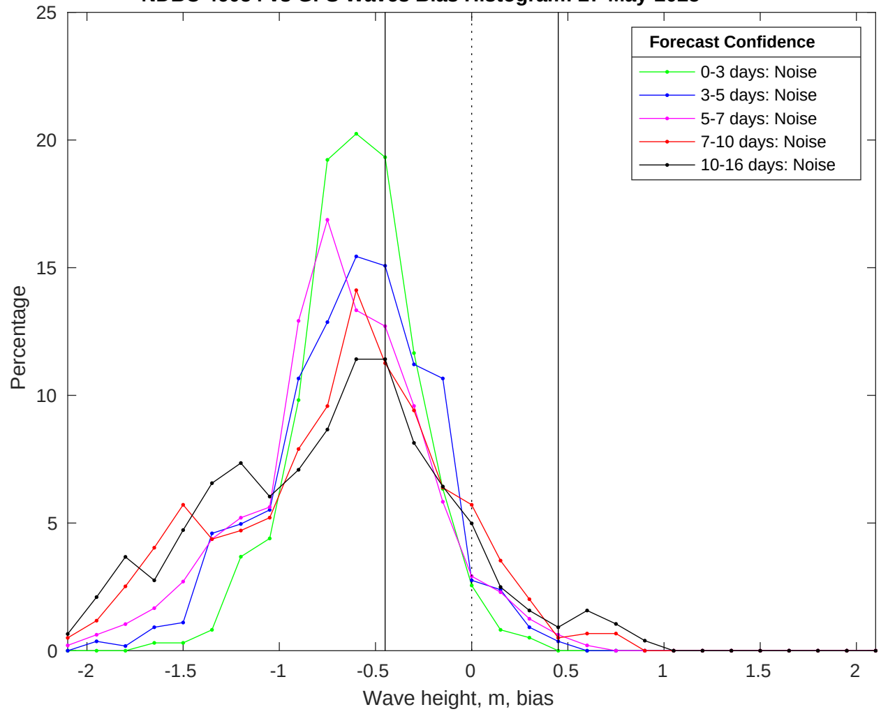
NDBC 46054 vs GFS Waves Bias Histogram: 27-May-2025
