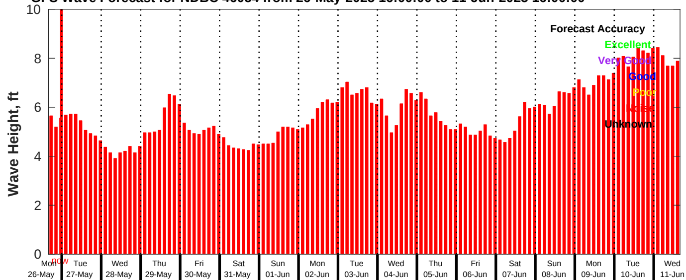
GFS Wave Forecast for NDBC 46054 from 26-May-2025 16:00:00 to 11-Jun-2025 16:00:00
