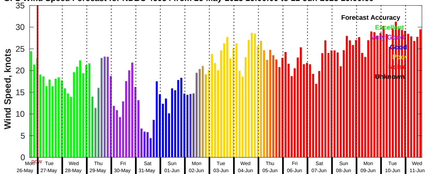
GFS Wind Speed Forecast for NDBC 46054 from 26-May-2025 16:00:00 to 11-Jun-2025 16:00:00
