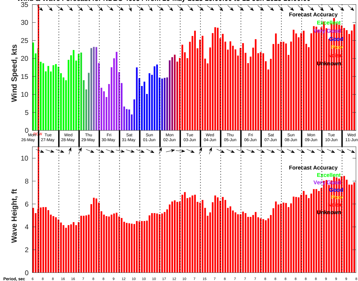
Wind & Wave Forecast for NDBC 46054 from 26-May-2025 16:00:00 to 11-Jun-2025 16:00:00
