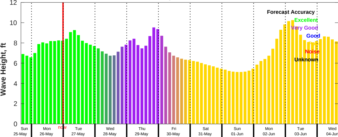
CMEMS Wave Forecast for NDBC 46069 from 25-May-2025 16:00:00 to 04-Jun-2025 16:00:00
