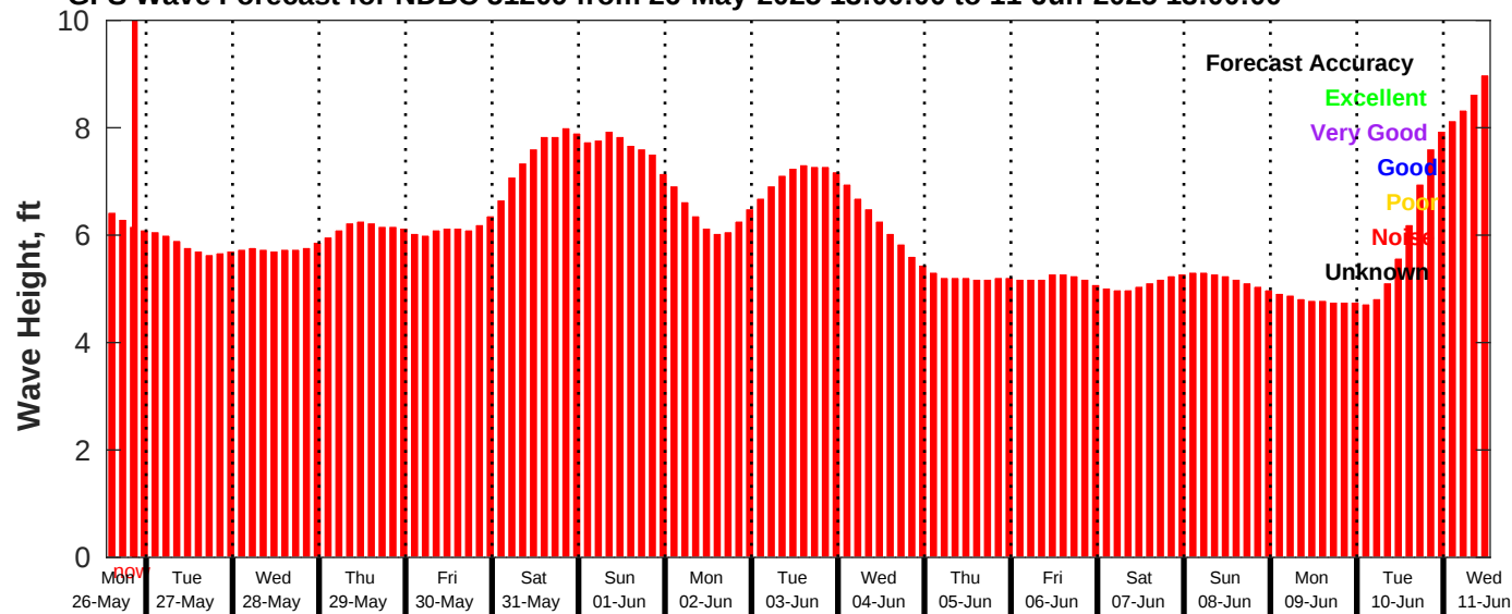
GFS Wave Forecast for NDBC 51209 from 26-May-2025 13:00:00 to 11-Jun-2025 13:00:00
