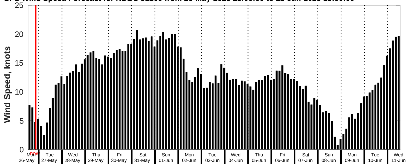
GFS Wind Speed Forecast for NDBC 51209 from 26-May-2025 13:00:00 to 11-Jun-2025 13:00:00
