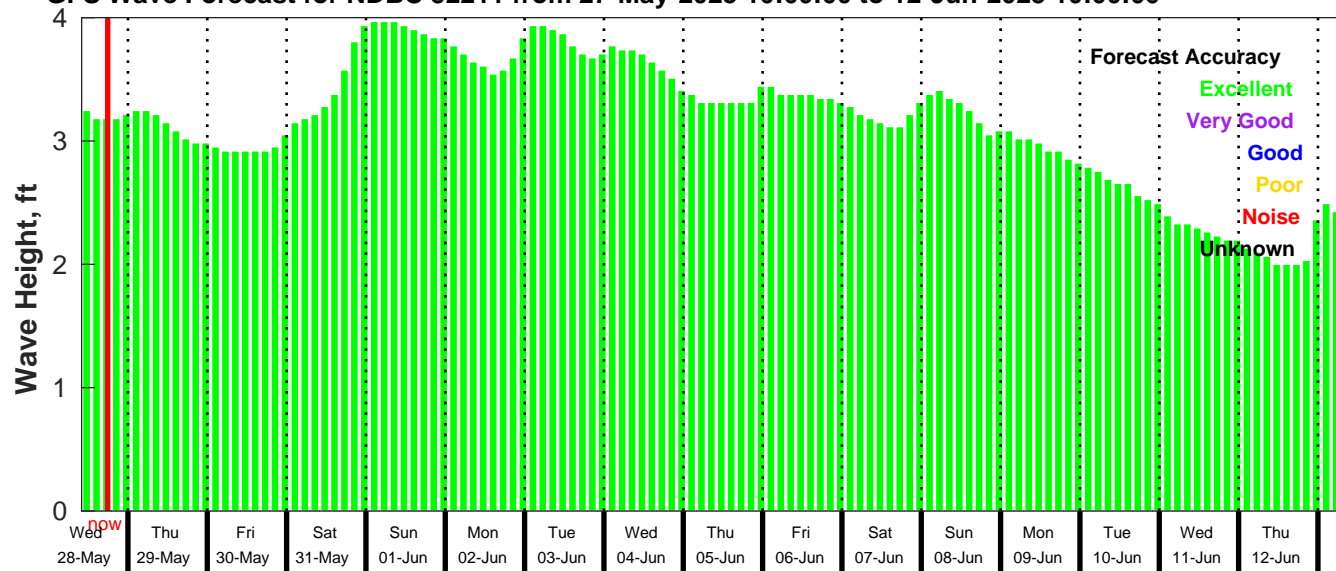
GFS Wave Forecast for NDBC 52211 from 27-May-2025 10:00:00 to 12-Jun-2025 10:00:00
