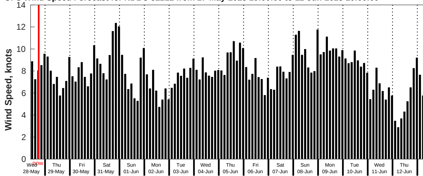
GFS Wind Speed Forecast for NDBC 52211 from 27-May-2025 10:00:00 to 12-Jun-2025 10:00:00
