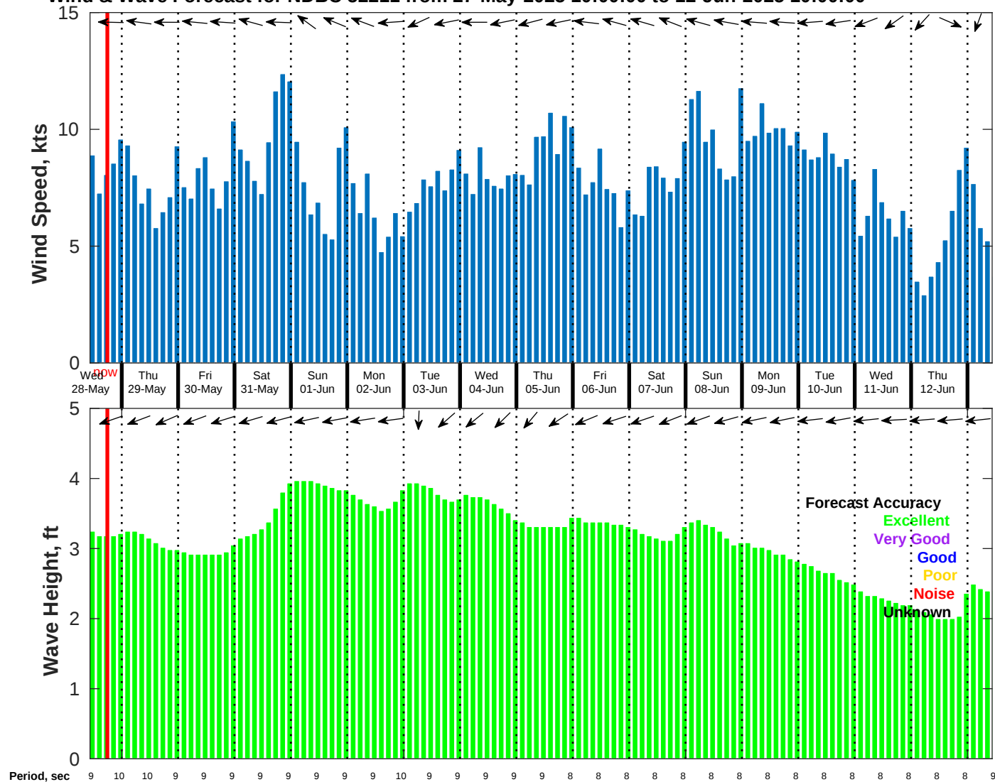
Wind & Wave Forecast for NDBC 52211 from 27-May-2025 10:00:00 to 12-Jun-2025 10:00:00
