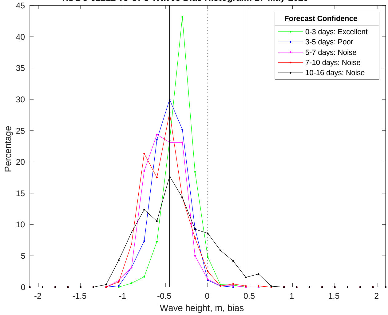
NDBC 52212 vs GFS Waves Bias Histogram: 27-May-2025
