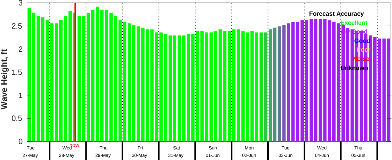
CMEMS Wave Forecast for NDBC 52212 from 26-May-2025 09:00:00 to 05-Jun-2025 09:00:00
