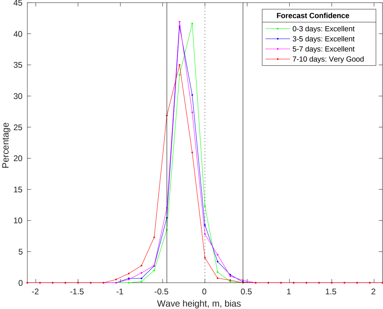
NDBC 52213 vs CMEMS Waves Bias Histogram: 27-May-2025
