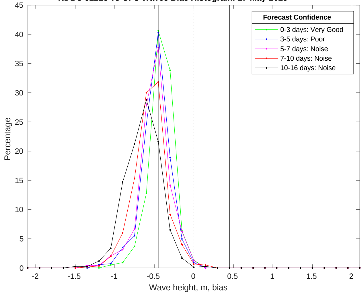
NDBC 52213 vs GFS Waves Bias Histogram: 27-May-2025
