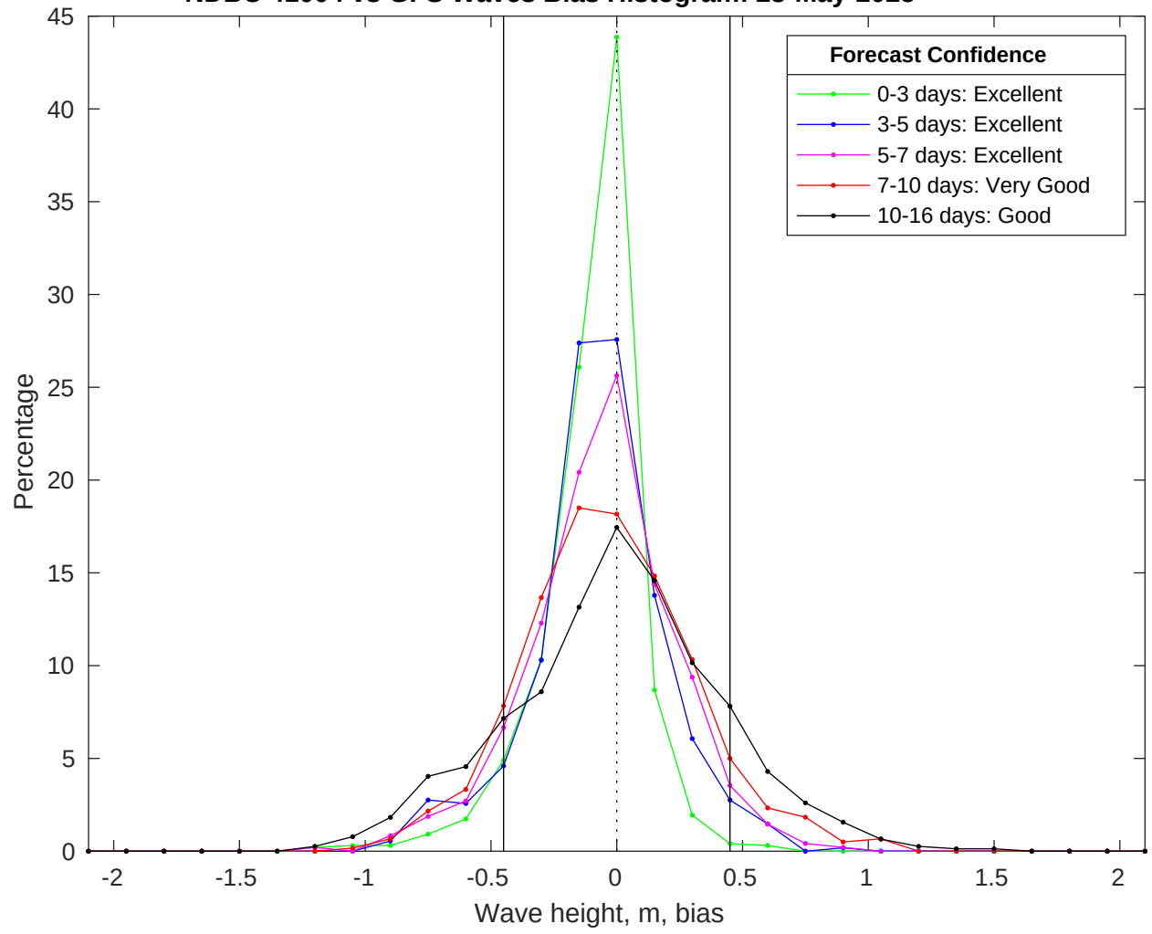
NDBC 41004 vs GFS Waves Bias Histogram: 28-May-2025
