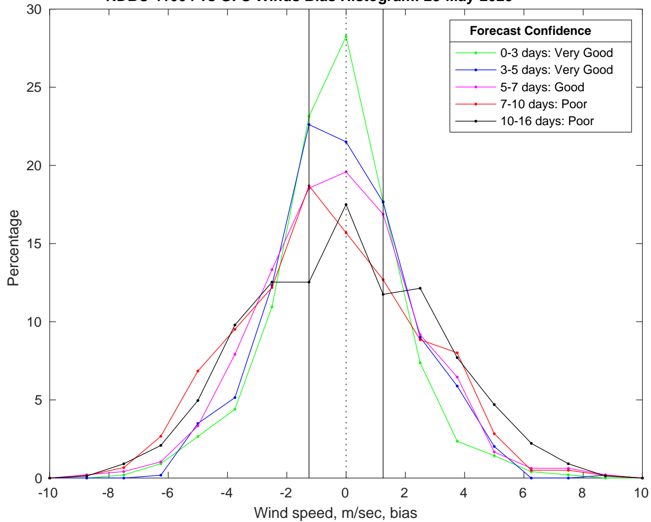
NDBC 41004 vs GFS Winds Bias Histogram: 28-May-2025
