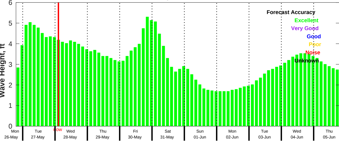
CMEMS Wave Forecast for NDBC 41004 from 26-May-2025 19:00:00 to 05-Jun-2025 19:00:00
