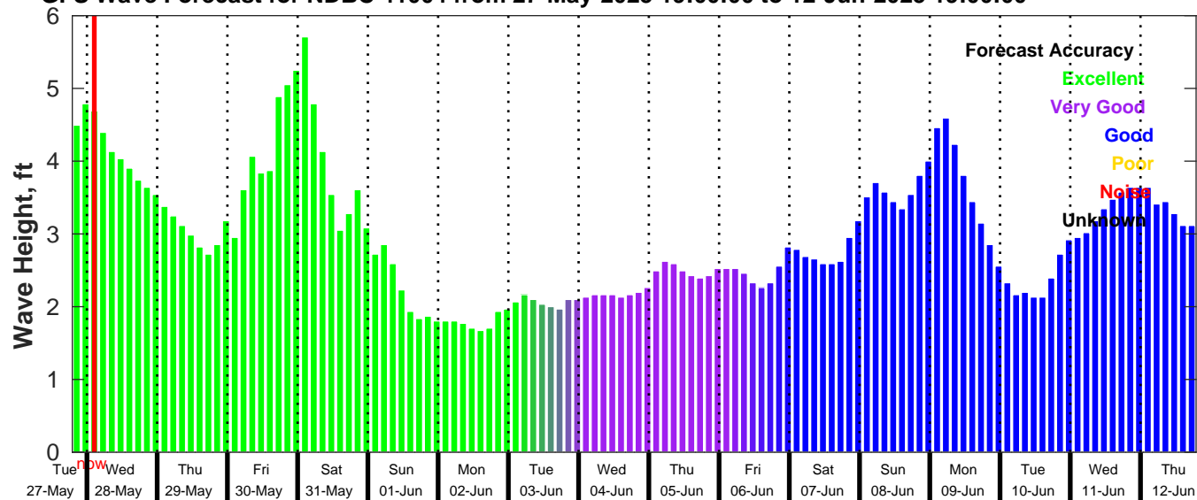
GFS Wave Forecast for NDBC 41004 from 27-May-2025 19:00:00 to 12-Jun-2025 19:00:00
