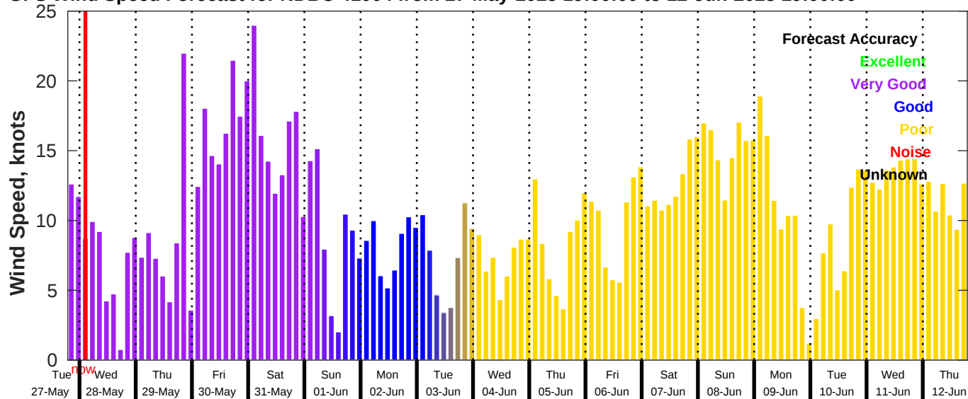
GFS Wind Speed Forecast for NDBC 41004 from 27-May-2025 19:00:00 to 12-Jun-2025 19:00:00
