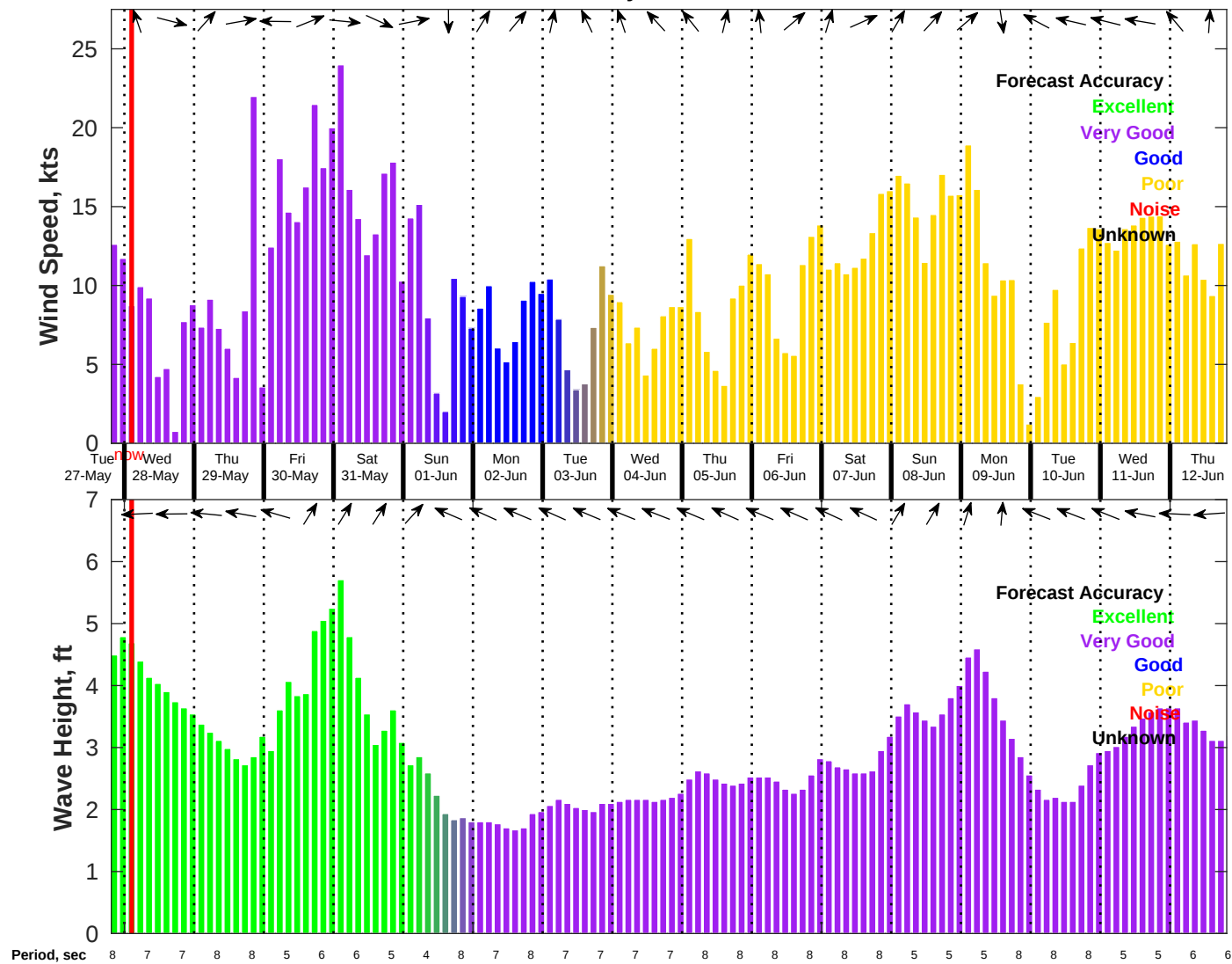
Wind & Wave Forecast for NDBC 41004 from 27-May-2025 19:00:00 to 12-Jun-2025 19:00:00
