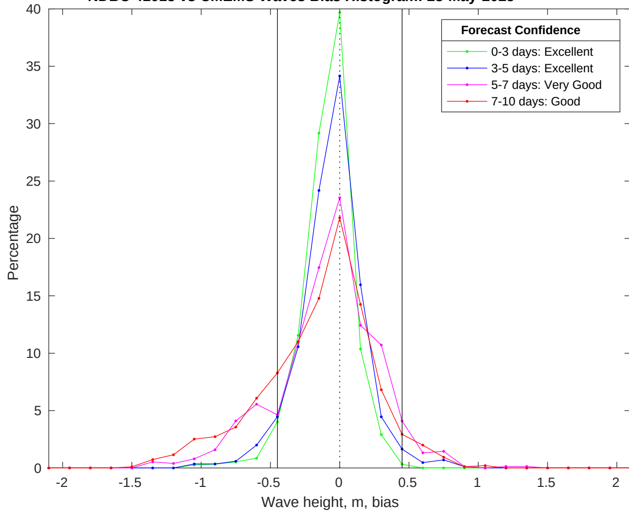
NDBC 41013 vs CMEMS Waves Bias Histogram: 28-May-2025
