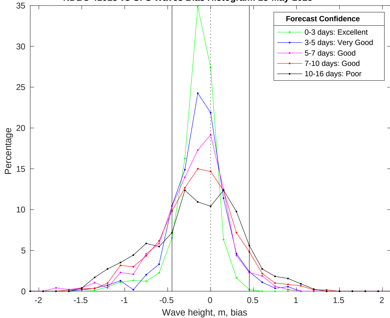
NDBC 41013 vs GFS Waves Bias Histogram: 28-May-2025
