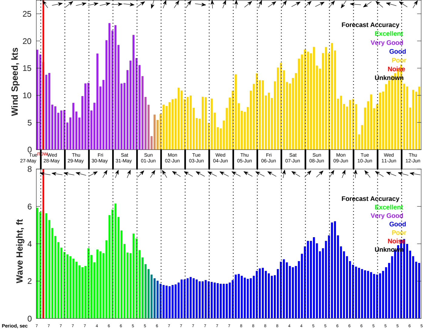
Wind & Wave Forecast for NDBC 41013 from 27-May-2025 19:00:00 to 12-Jun-2025 19:00:00
