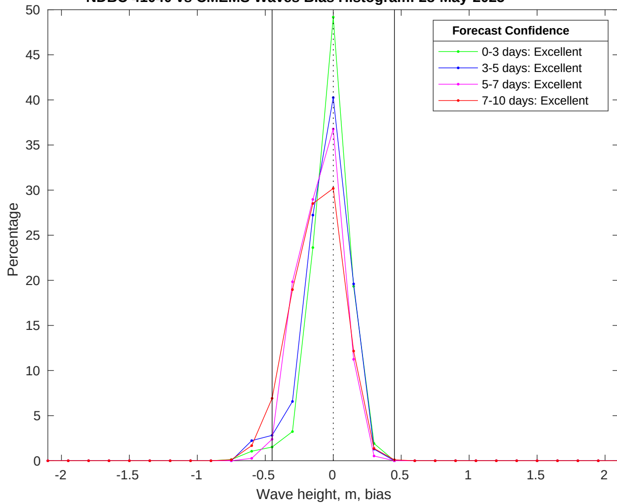
NDBC 41040 vs CMEMS Waves Bias Histogram: 28-May-2025
