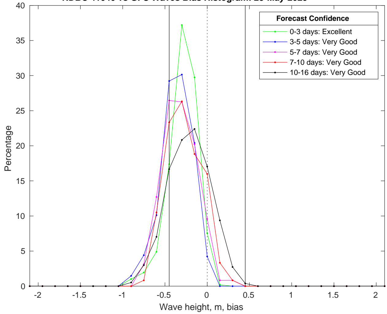
NDBC 41040 vs GFS Waves Bias Histogram: 28-May-2025
