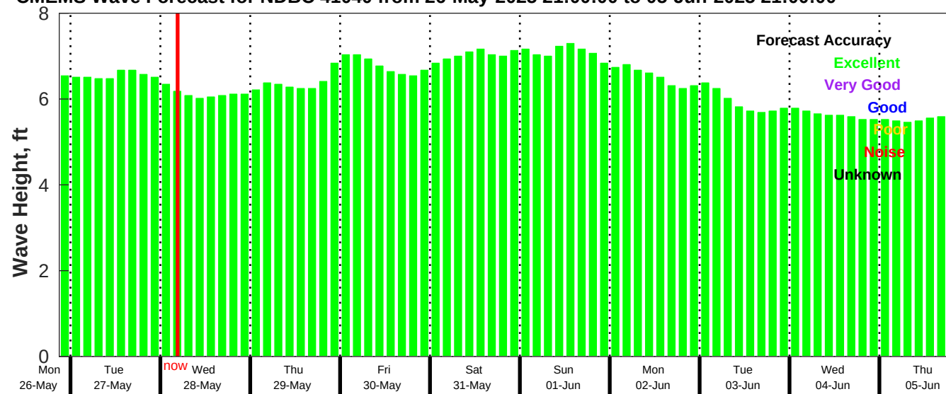
CMEMS Wave Forecast for NDBC 41040 from 26-May-2025 21:00:00 to 05-Jun-2025 21:00:00
