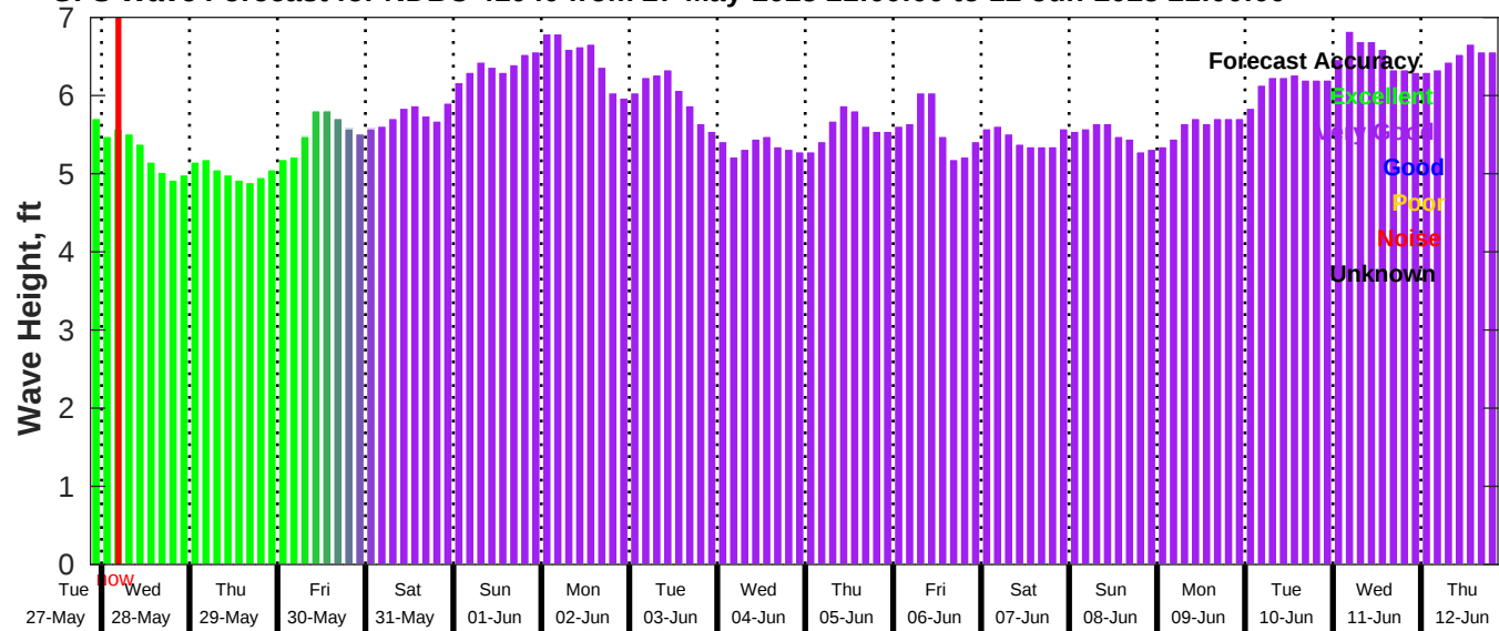
GFS Wave Forecast for NDBC 41040 from 27-May-2025 21:00:00 to 12-Jun-2025 21:00:00
