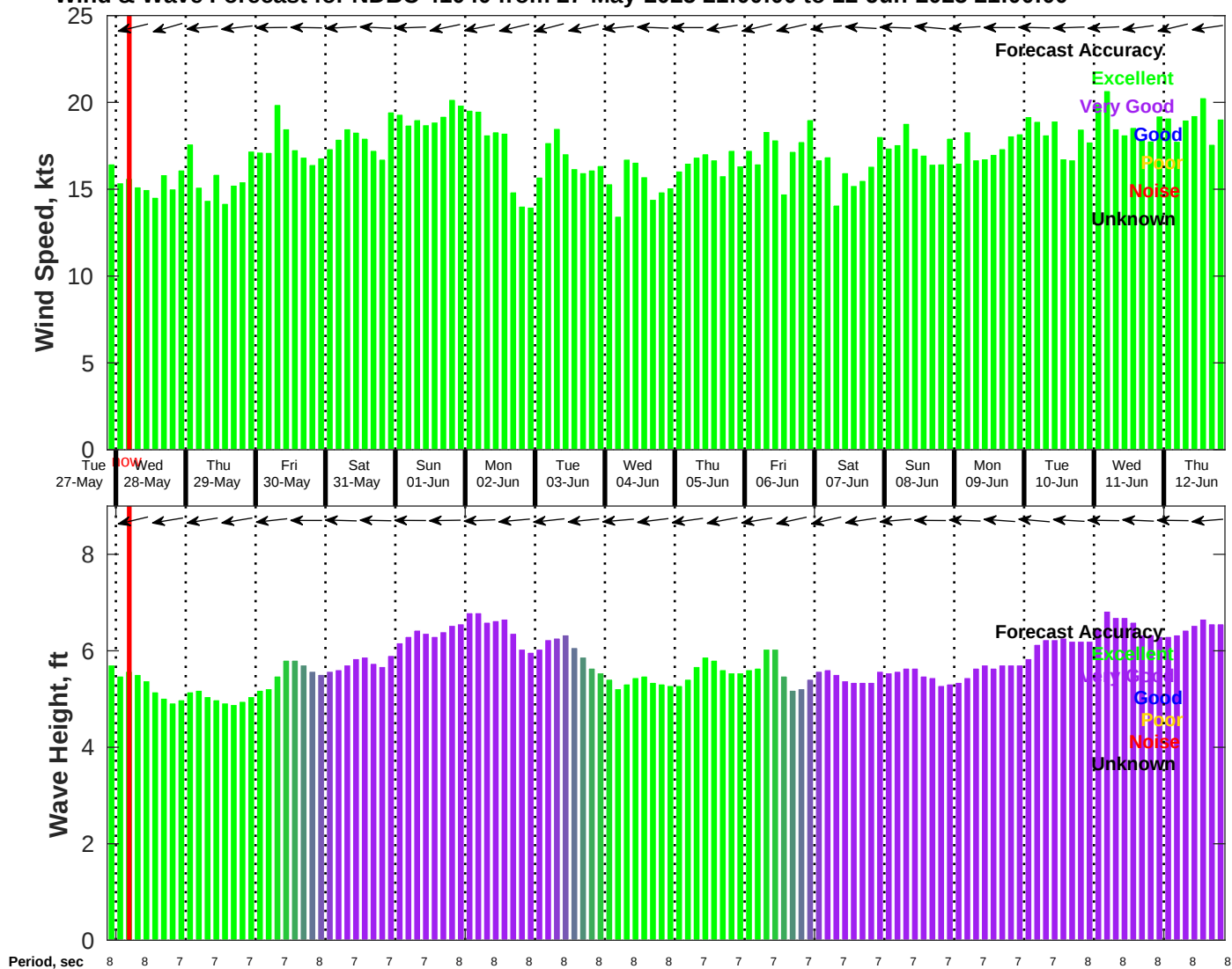
Wind & Wave Forecast for NDBC 41040 from 27-May-2025 21:00:00 to 12-Jun-2025 21:00:00
