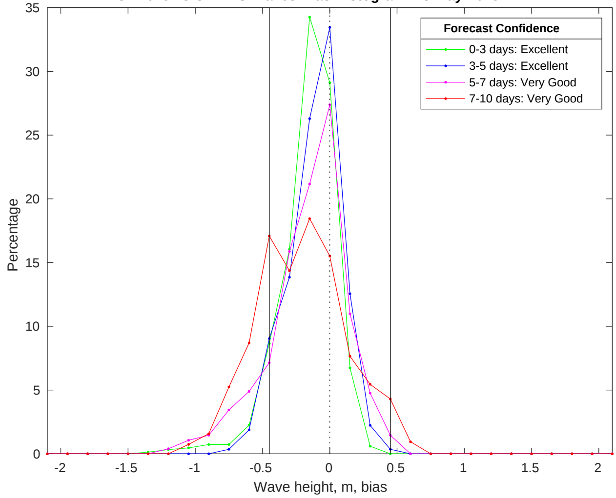
NDBC 42019 vs CMEMS Waves Bias Histogram: 28-May-2025
