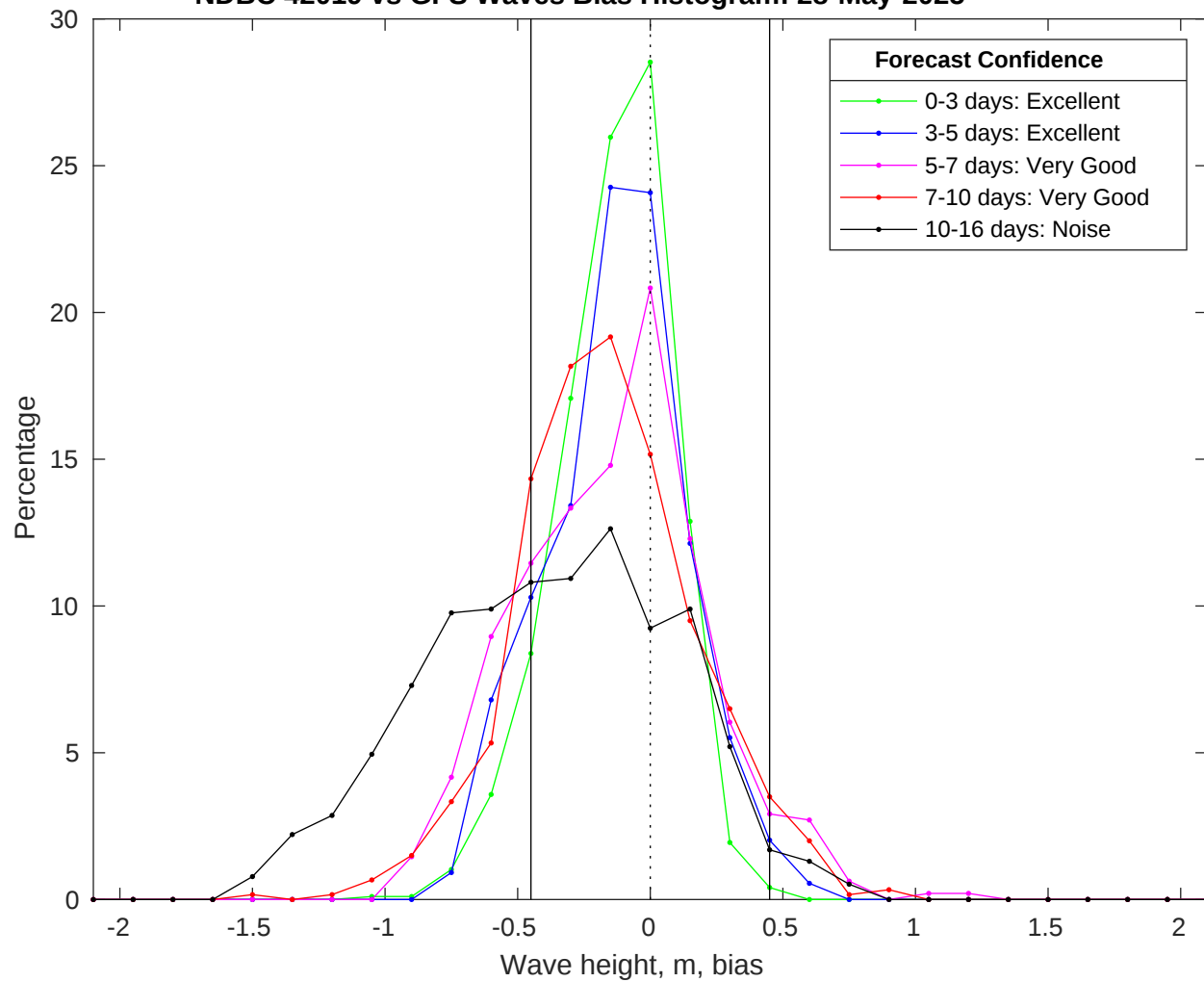
NDBC 42019 vs GFS Waves Bias Histogram: 28-May-2025
