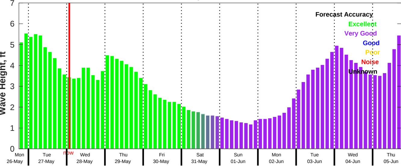
CMEMS Wave Forecast for NDBC 42019 from 26-May-2025 18:00:00 to 05-Jun-2025 18:00:00
