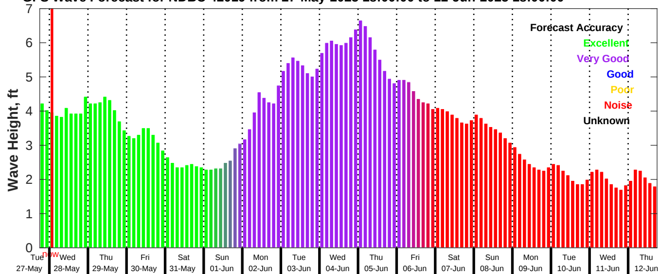
GFS Wave Forecast for NDBC 42019 from 27-May-2025 18:00:00 to 12-Jun-2025 18:00:00
