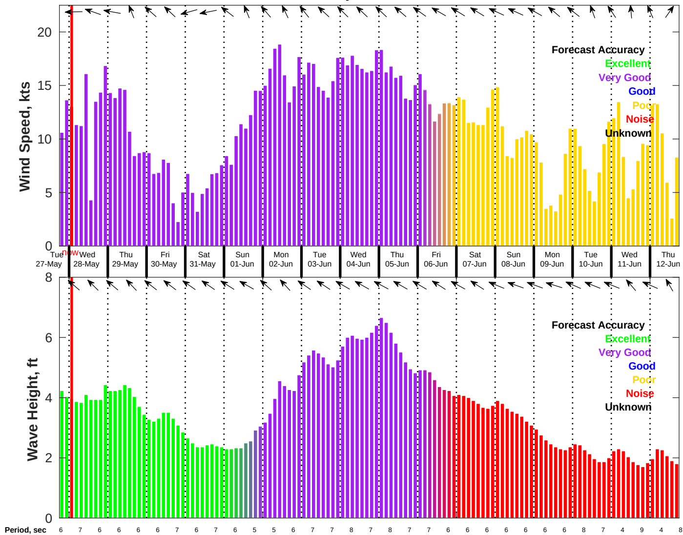
Wind & Wave Forecast for NDBC 42019 from 27-May-2025 18:00:00 to 12-Jun-2025 18:00:00
