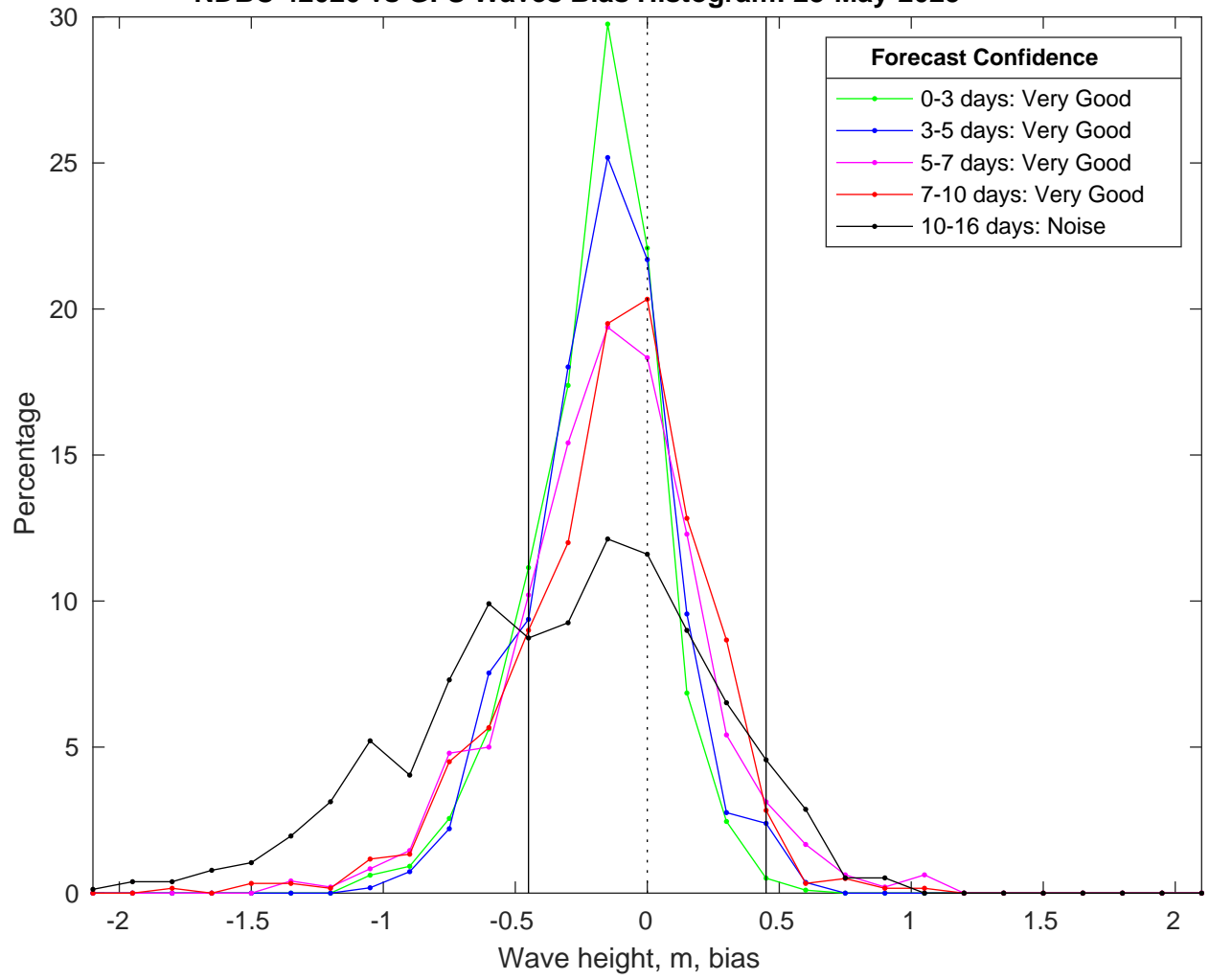
NDBC 42020 vs GFS Waves Bias Histogram: 28-May-2025
