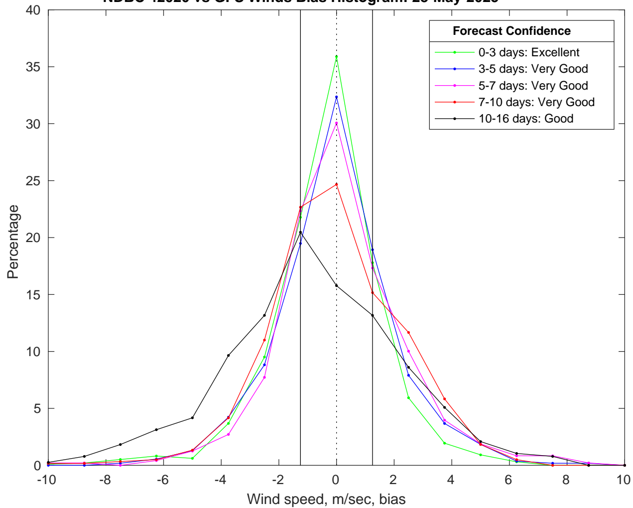
NDBC 42020 vs GFS Winds Bias Histogram: 28-May-2025
