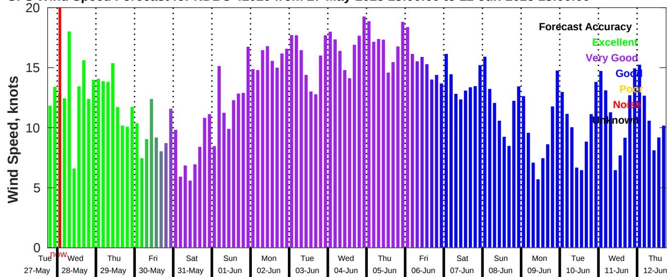
GFS Wind Speed Forecast for NDBC 42020 from 27-May-2025 18:00:00 to 12-Jun-2025 18:00:00
