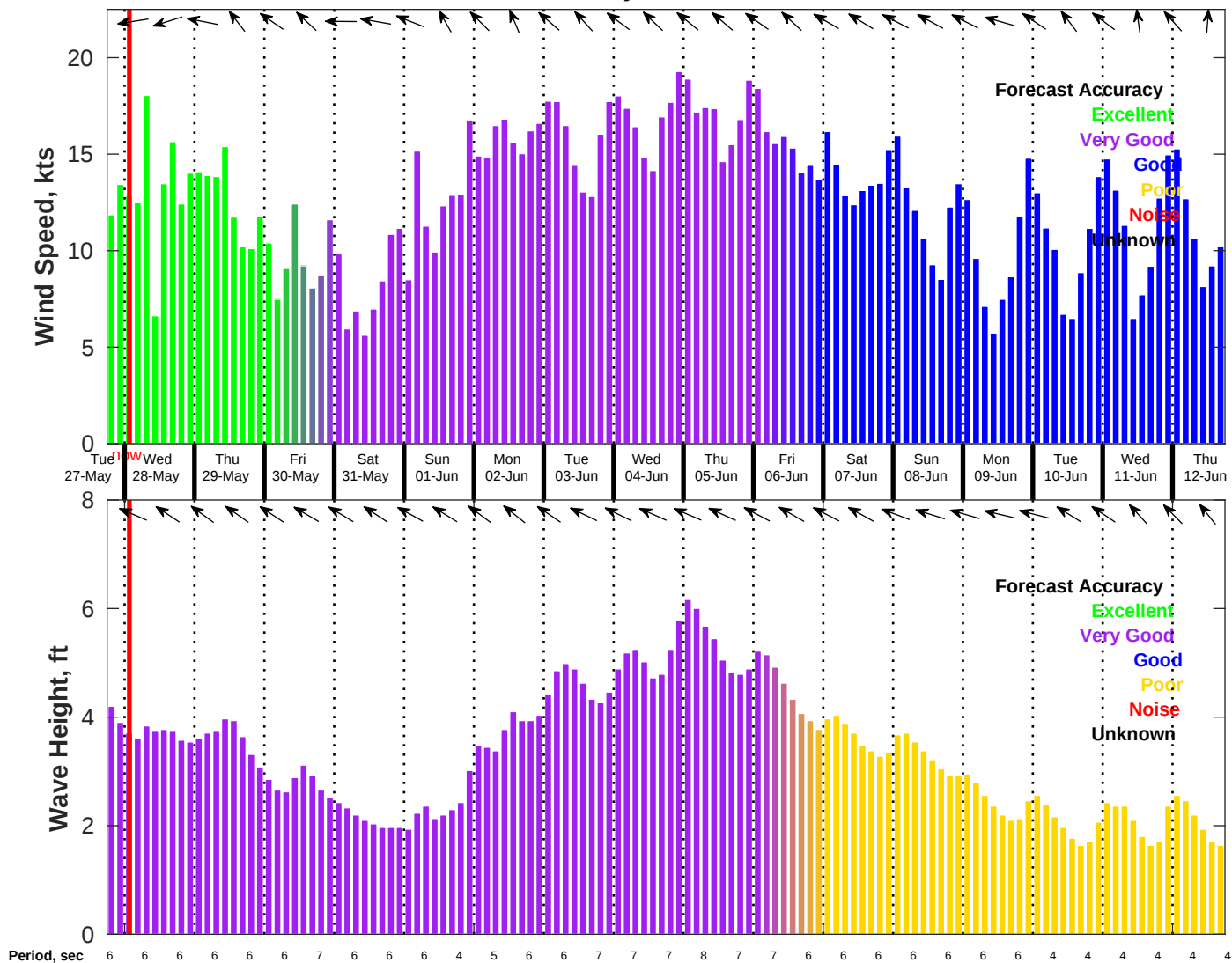
Wind & Wave Forecast for NDBC 42020 from 27-May-2025 18:00:00 to 12-Jun-2025 18:00:00
