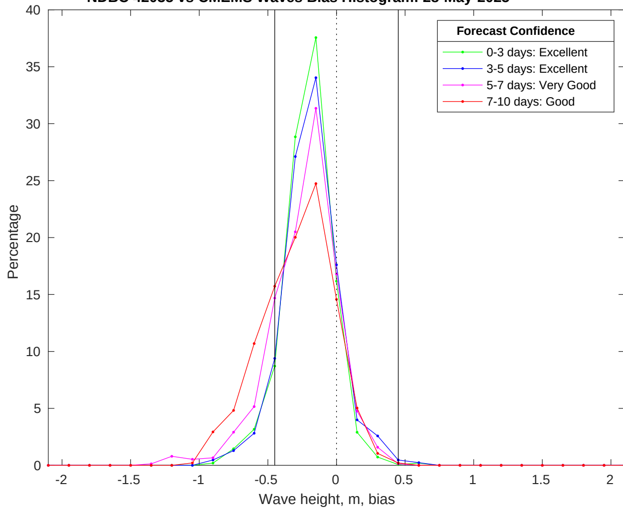
NDBC 42035 vs CMEMS Waves Bias Histogram: 28-May-2025
