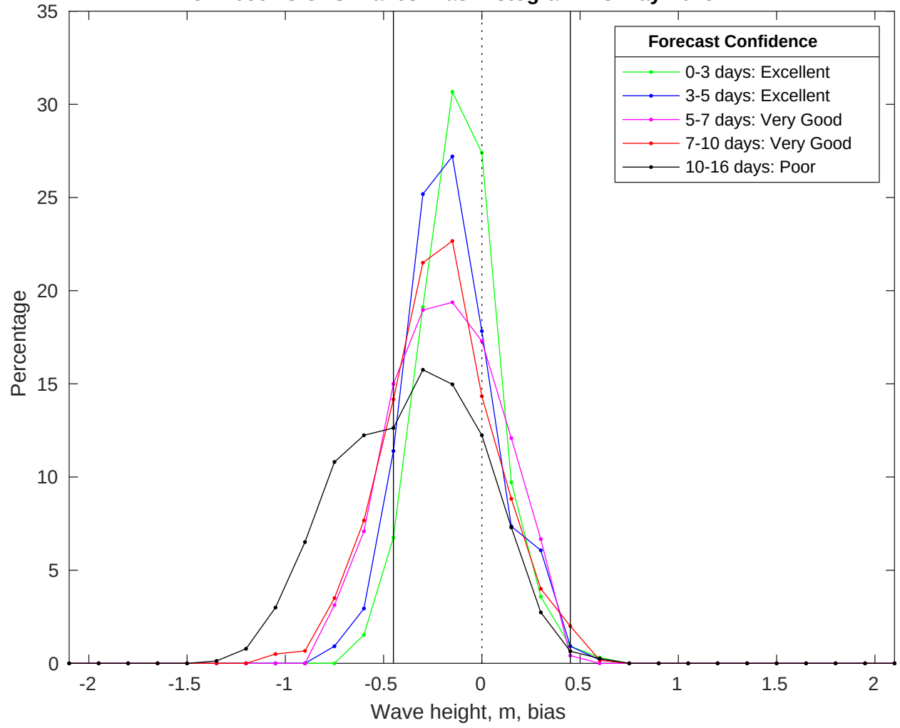
NDBC 42035 vs GFS Waves Bias Histogram: 28-May-2025
