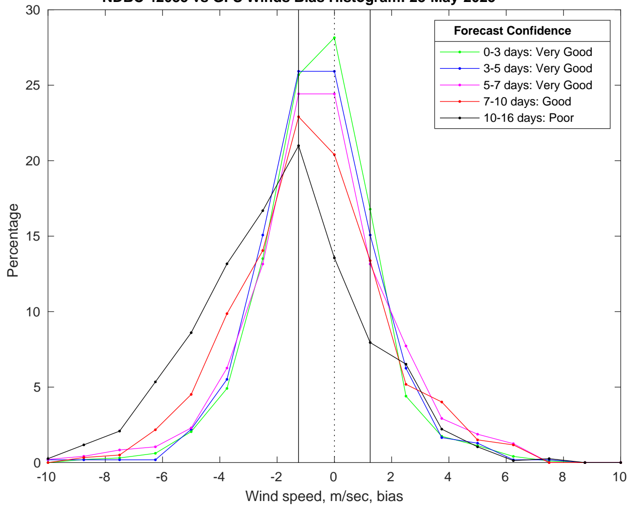
NDBC 42035 vs GFS Winds Bias Histogram: 28-May-2025
