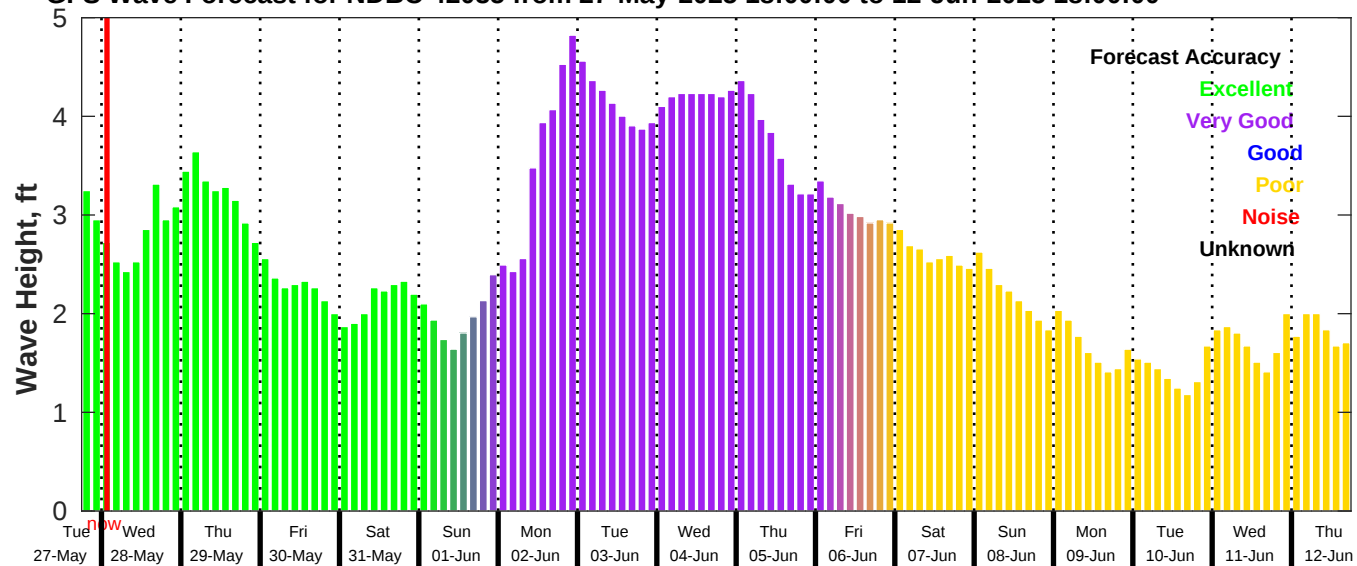
GFS Wave Forecast for NDBC 42035 from 27-May-2025 18:00:00 to 12-Jun-2025 18:00:00
