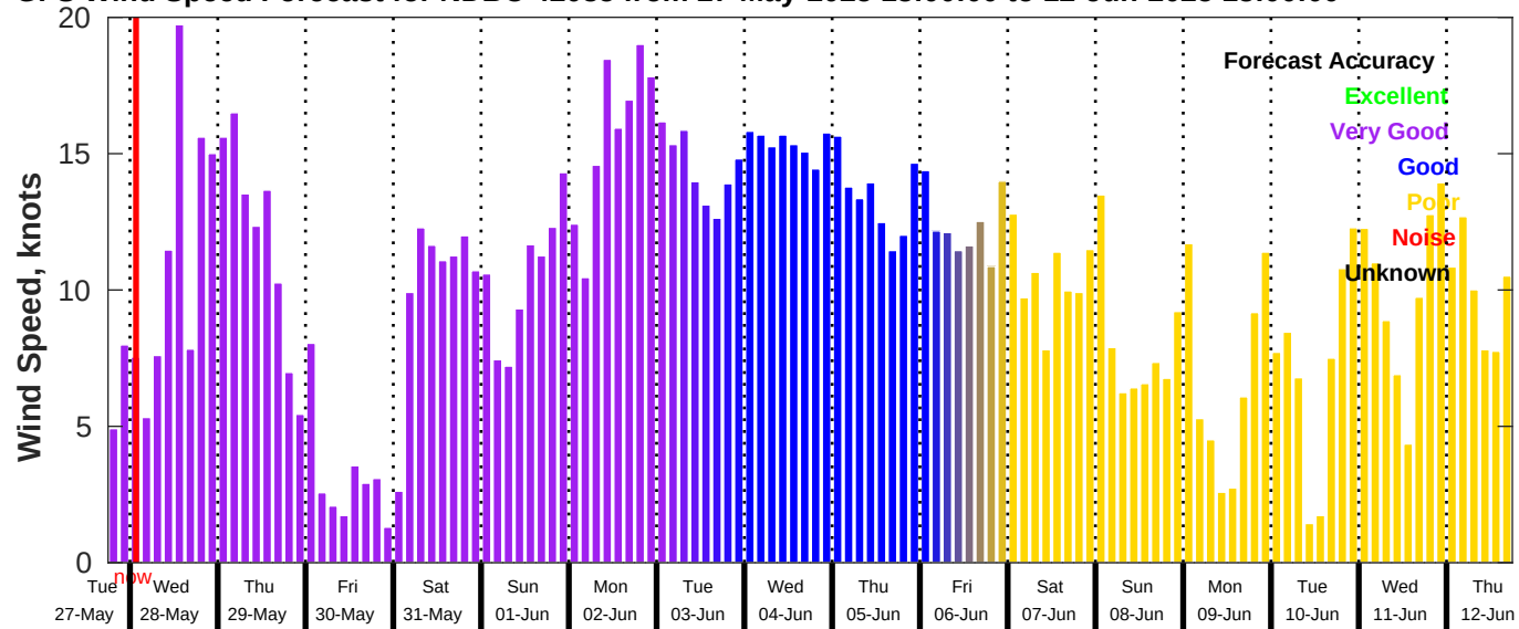
GFS Wind Speed Forecast for NDBC 42035 from 27-May-2025 18:00:00 to 12-Jun-2025 18:00:00
