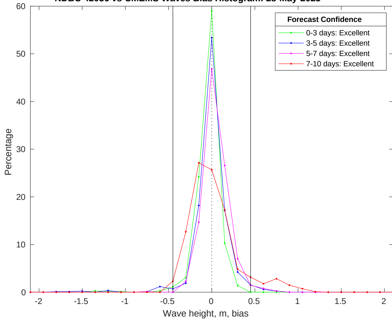
NDBC 42036 vs CMEMS Waves Bias Histogram: 28-May-2025
