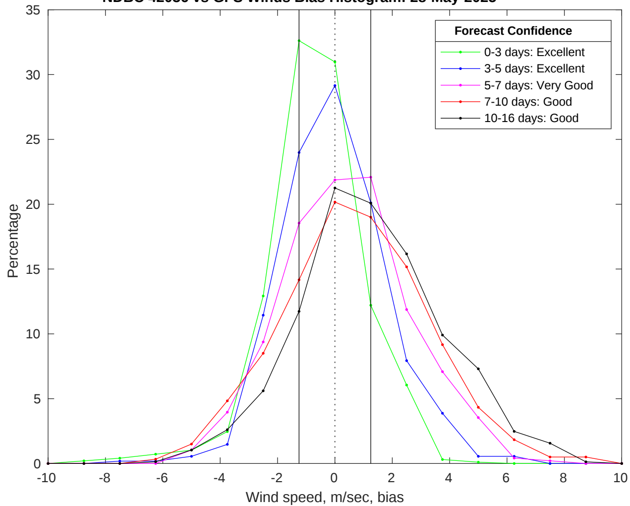
NDBC 42036 vs GFS Winds Bias Histogram: 28-May-2025
