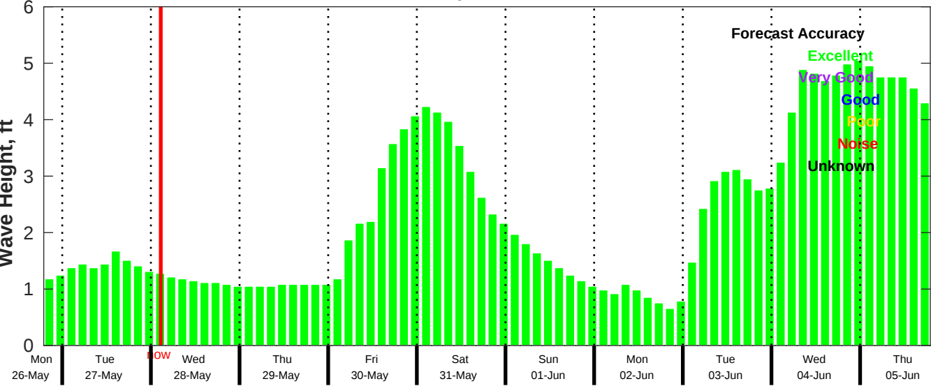
CMEMS Wave Forecast for NDBC 42036 from 26-May-2025 19:00:00 to 05-Jun-2025 19:00:00
