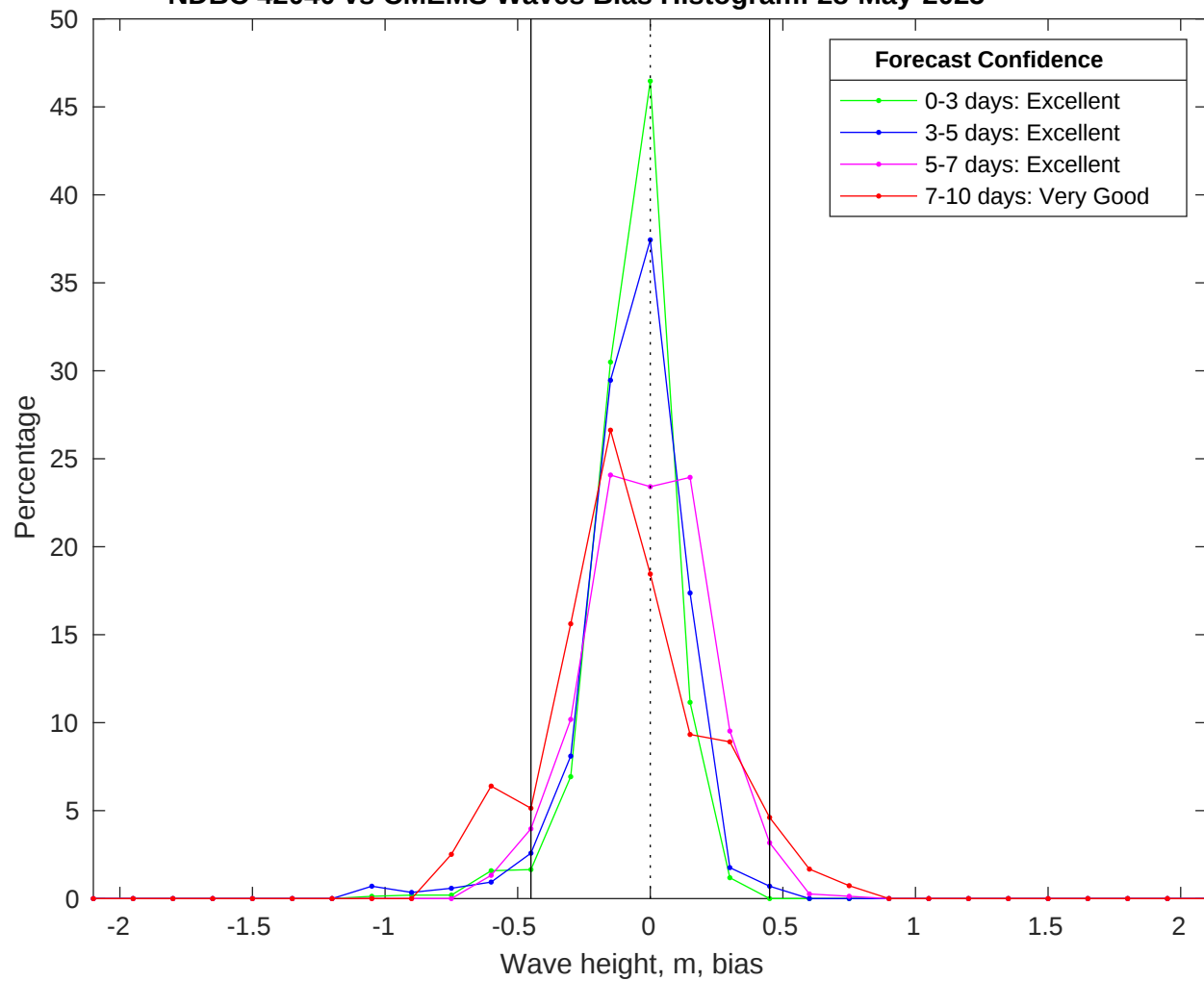
NDBC 42040 vs CMEMS Waves Bias Histogram: 28-May-2025
