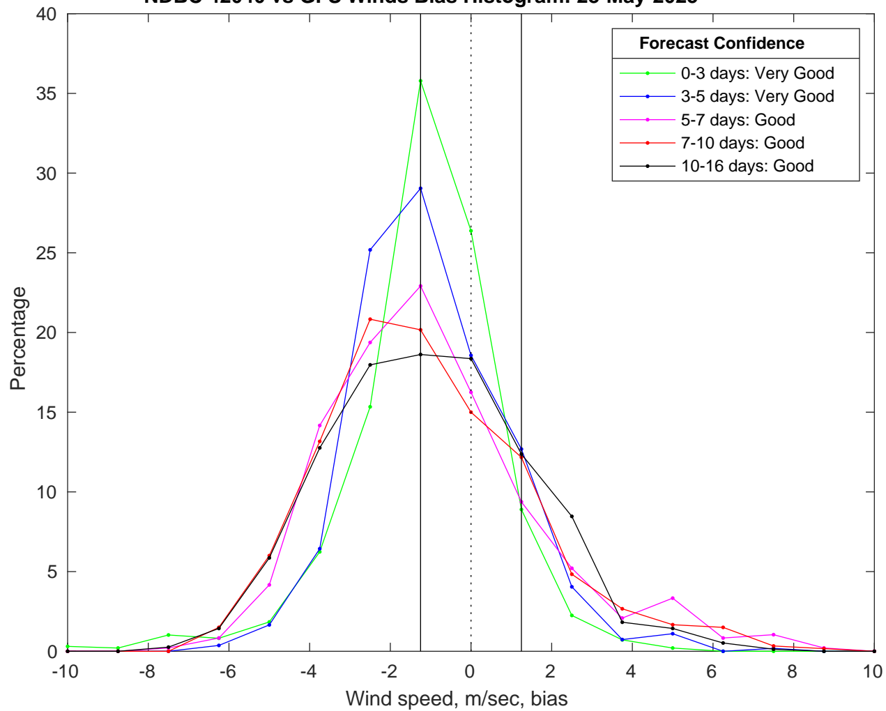
NDBC 42040 vs GFS Winds Bias Histogram: 28-May-2025
